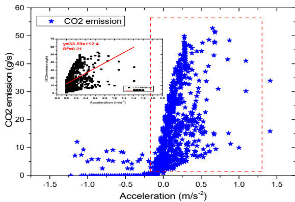
Figure 5 CO 2 emission versus vehicle acceleration for trailer tractor
