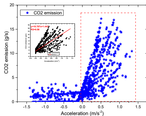
Figure 3 CO2 emission versus vehicle acceleration for city bus
