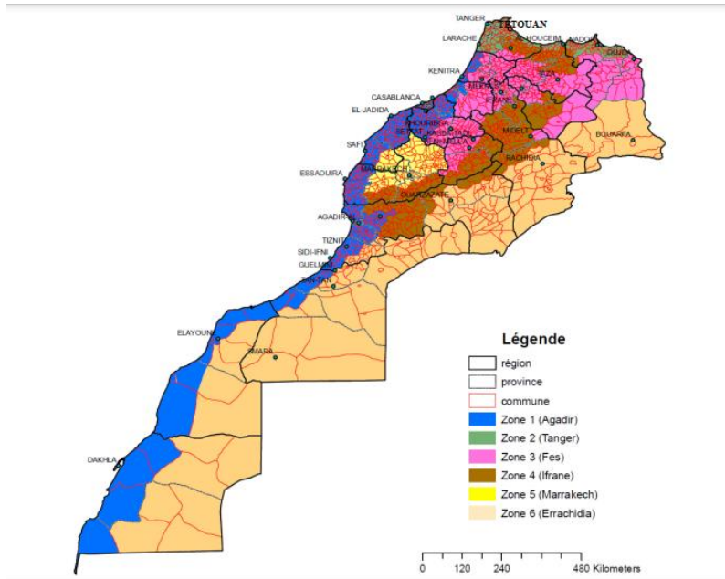
Fig. 2: Distribution of climate zones in Morocco [5]
