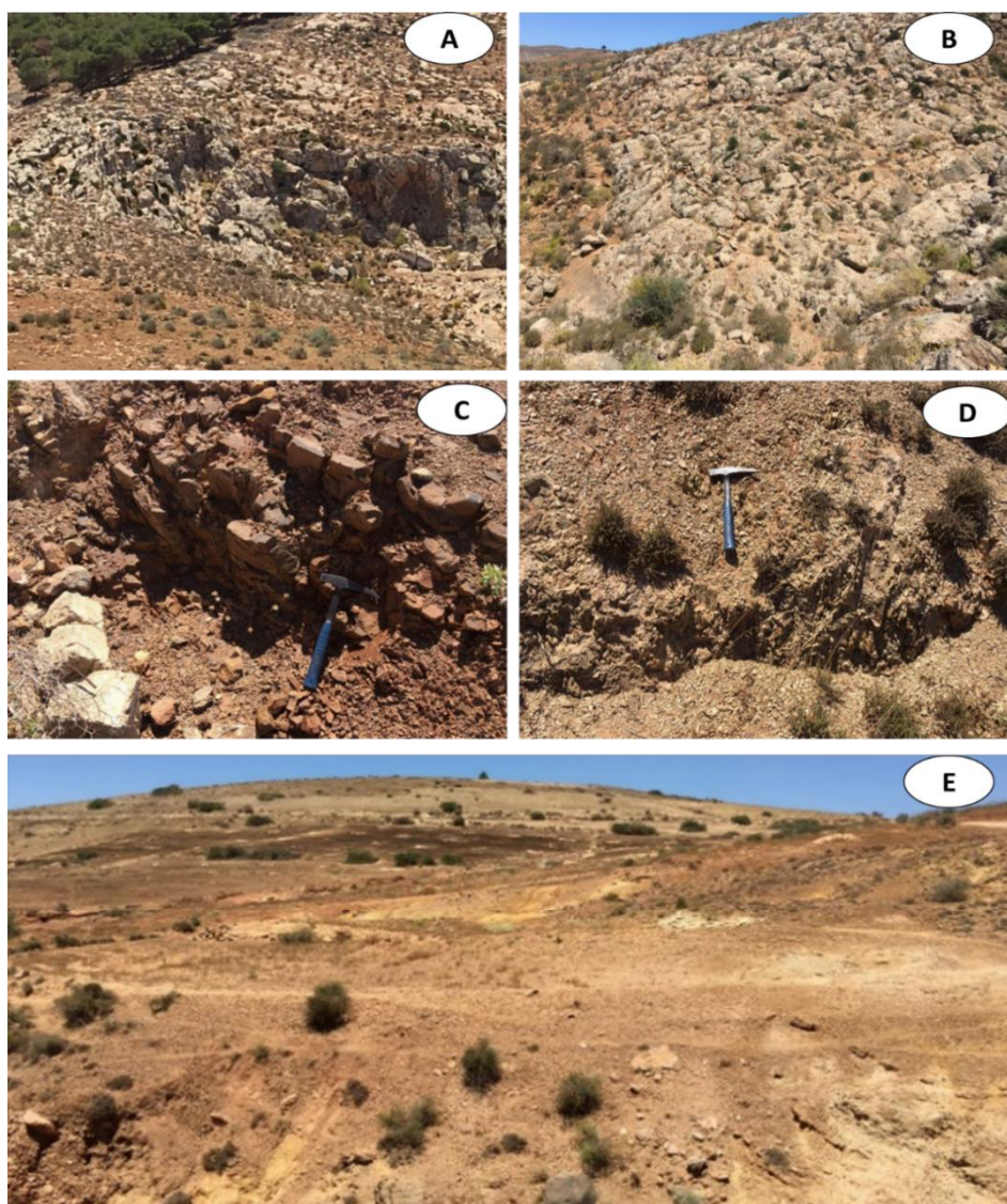
Fig 5. lithostratigraphic facies of the Jbel Harcha unit: A and B Jurassic carbonate; C and D: Cretaceous shale; E Neogene marl unconformity on Jurassic marl and limestone
