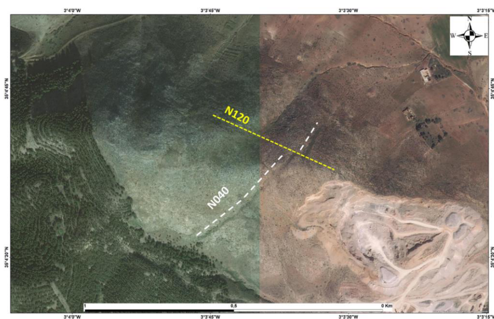
Fig 8. satellite image shows the intersection of faults N040 and N120
