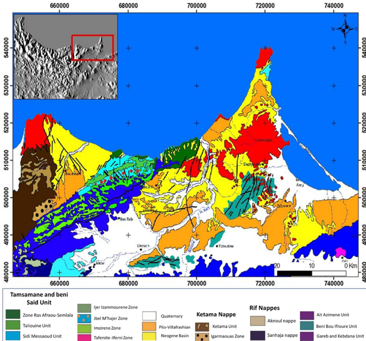
Fig 1. structural diagram of Rif shows the location of the study area (extracted from the geological map of Zeghanghane) [8]
