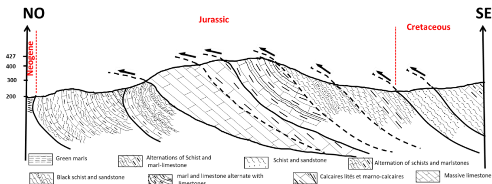
Fig 6. Schematic geological section NW-SE at the level of jbel Harcha
