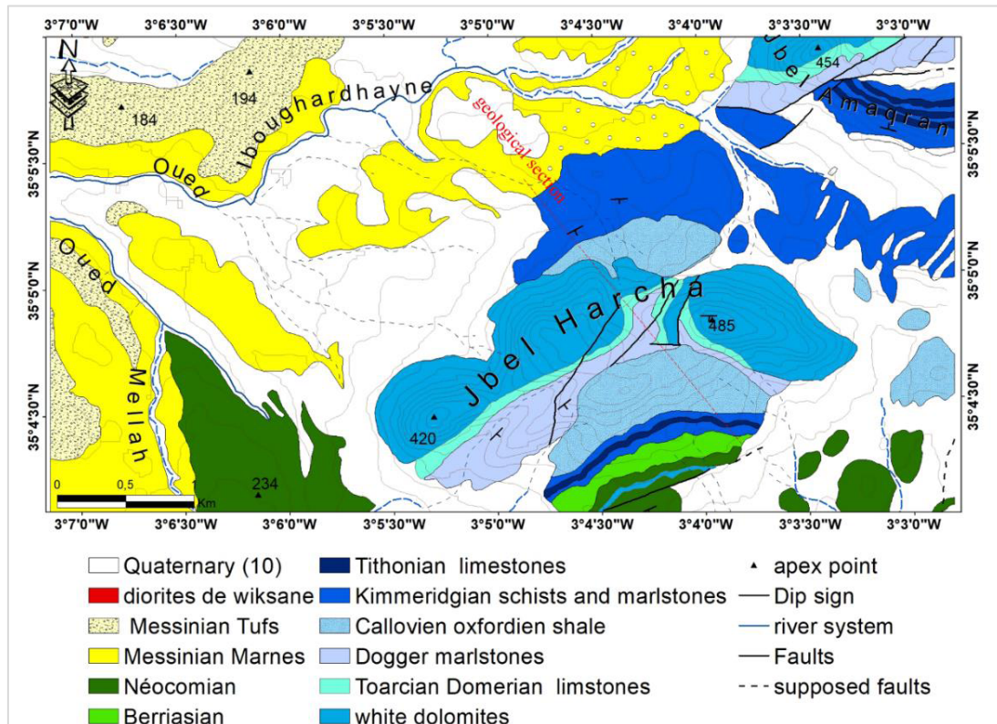
Fig 3. Geological map of Jbel Harcha, extracted from the geological map of Zeghanghane at 1/50000, modified
