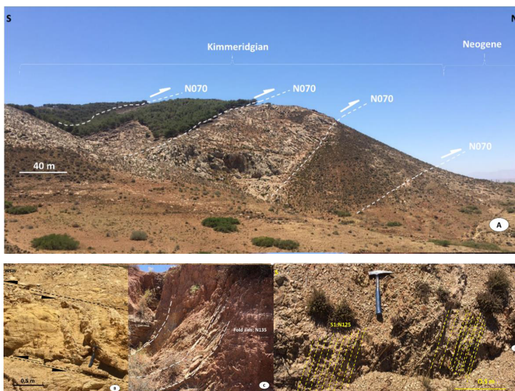
Fig 7. A) N070 thrusts in the Jurassic carbonates; B) crossover shows that there is a sinister displacement; C) folds related to the thrusts; D) schistosity axes
