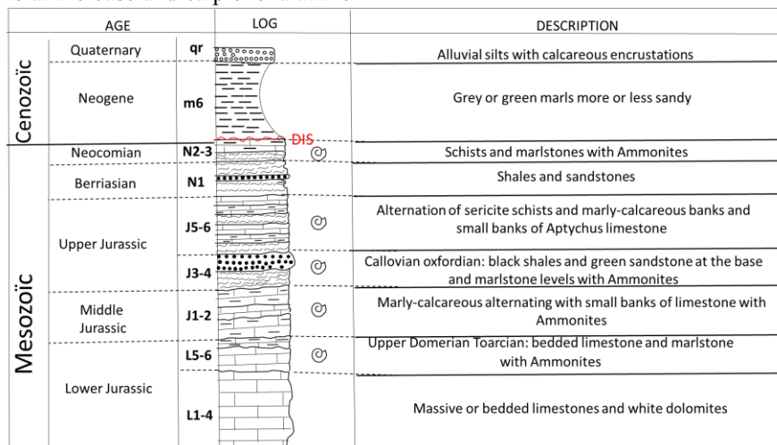
Fig 4. Stratigraphic log of the Jbel Harcha unit
