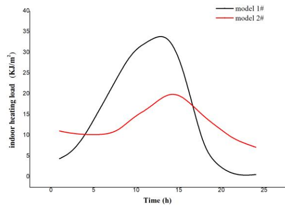
Fig. 13 Change of indoor heating load when PCM is 8°C
