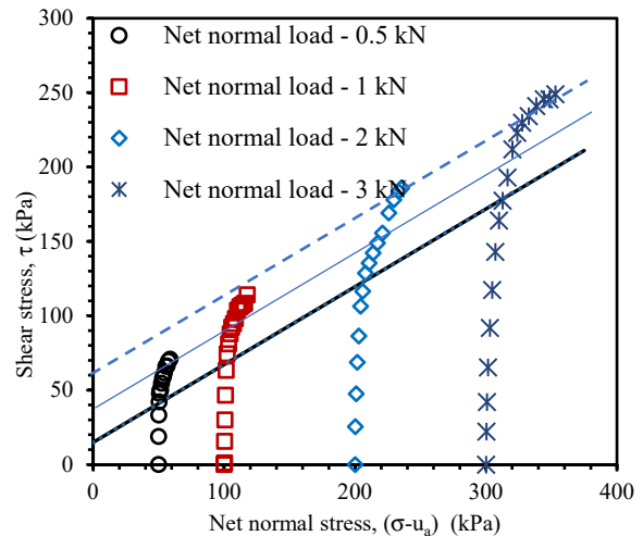
Fig. 5. Stress paths for unsaturated direct shear tests for CDG at 50 kPa matric suction (data from Hossain and Yin [19]).
