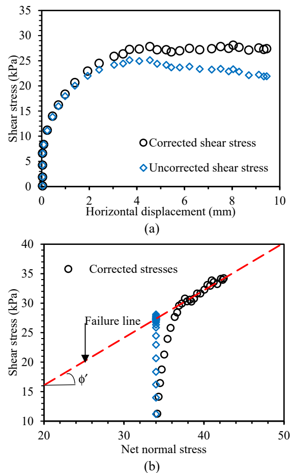
Fig. 3. Illustration of the use of stress path to interpret constant suction direct shear tests from Han [48] with no peak shear stress.
