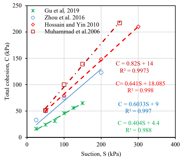
Fig. 6. Re-interpreted data for case of different slopes.
