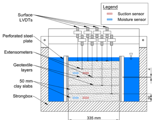
Fig. 4. Model layout
