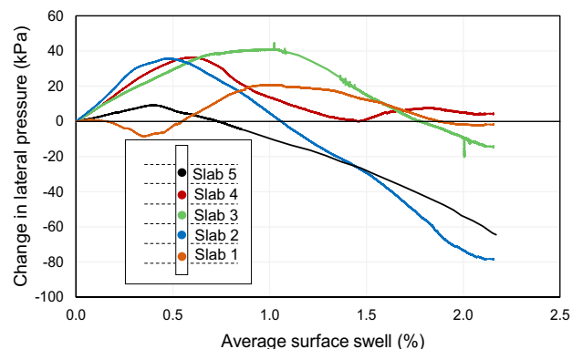
Fig. 7. Changes in lateral pressure against pile shaft
