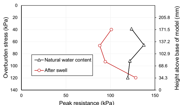
Fig. 6. Comparison of pull-out capacity of short length piles
