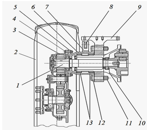
Fig. 2. A mechanism for changing the clearance of the rear axle of the tractor, rear view: 1 - semi-axle; 2 - driving wheel; 3 - a body of additional final drive; 4, 11 - fasteners; 5 - end flange; 6 - clip; 7 - lever; 8 - hydraulic cylinder rod; 9 - suspension bracket for hanging devices; 10 - semi-axle sleeves; 12 - fixing flange; 13 - needle bearings
