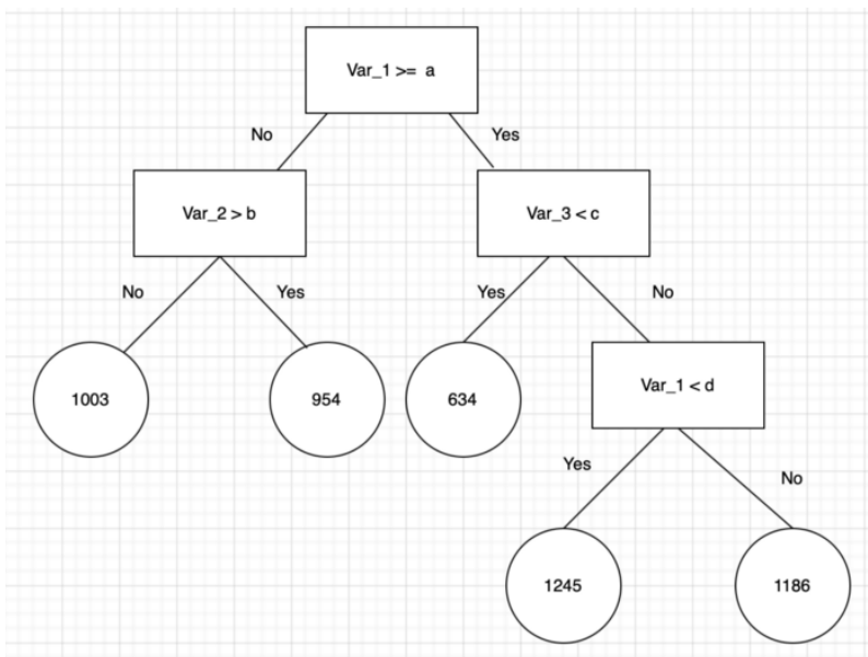
Fig 2. Decision tree
