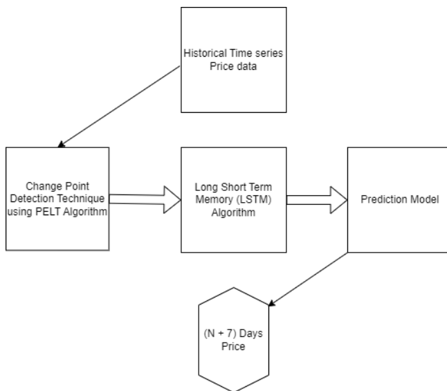
Fig.1: System architecture
