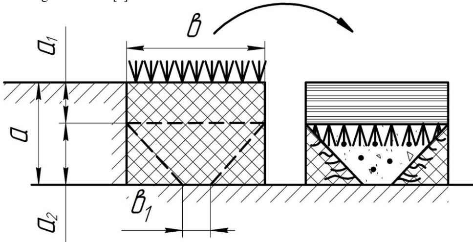
\alpha – tillage depth; \alpha_1 - depth of the top root-inhabited soil layer; \alpha_2 - depth of the lower tilled soil layer, \beta - width of the plow bottom; \beta_1 - width of the mouldboardless ripper
