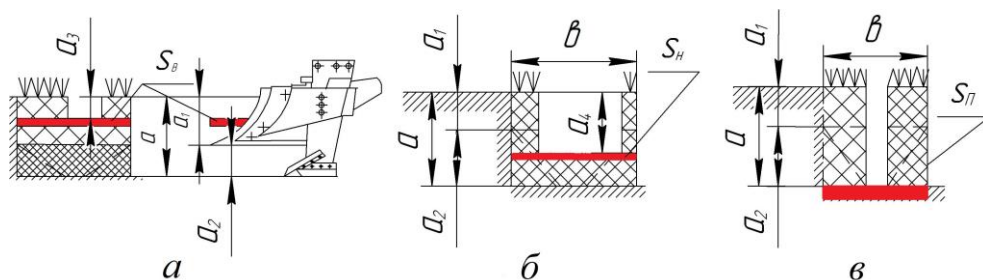
S_B, S_H, S_{\Pi} - sampling levels, respectively, the top, lower tilled and subsurface layer
