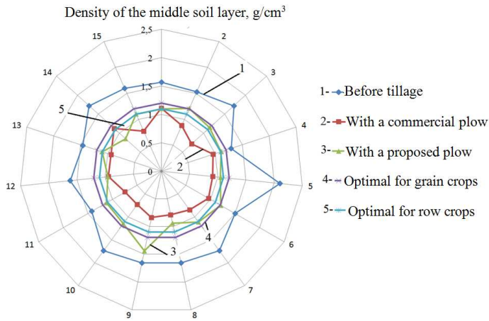
Fig. 8. Density of the lower cultivated arable soil layer before and after tillage.
