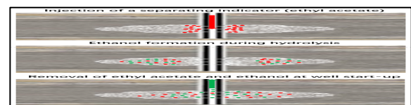
FIG. 2 Schematic diagram of single-well tracer testing
