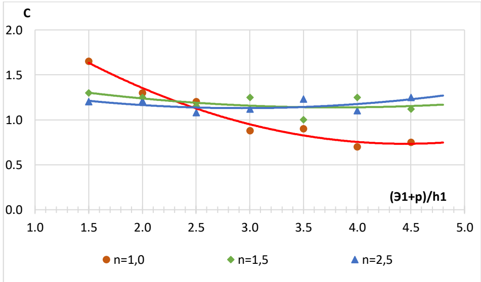
Fig.4. Determination of average horizontal stresses for research scheme.
