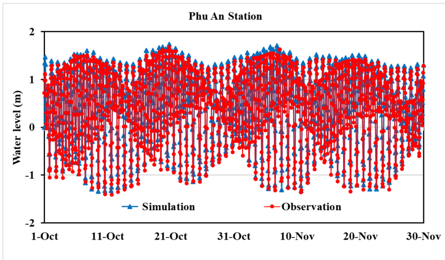
Fig. 6. Water level in Phu An station, time measurement from October 1 to November 30, 2013
