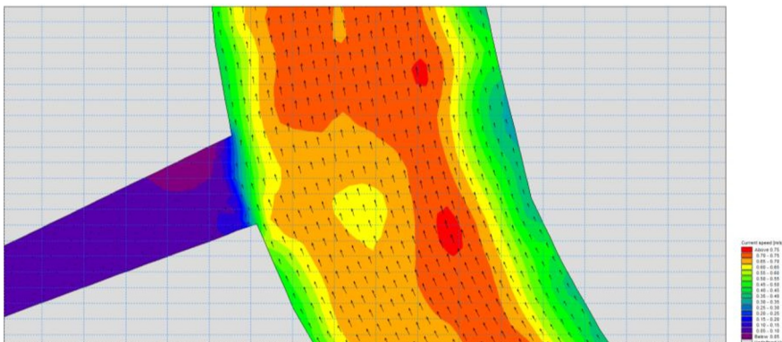
Fig. 12. Distribution of flow velocity in high water during high tide.
