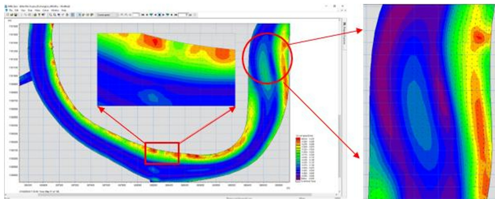
Fig. 8. Distribution of flow velocity at end of low tide and beginning of high tide.
