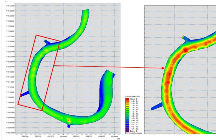
Fig. 11. Distribution of flow velocity during low tide in April-May.
