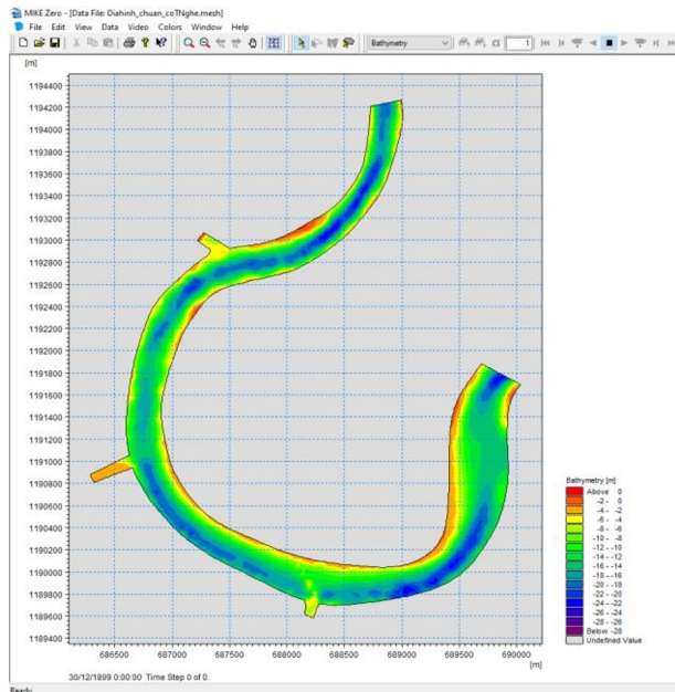
Fig. 4. Topography of Sai Gon River section from Sai Gon Bridge to Cape Diamond.
