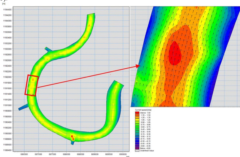
Fig. 10. Distribution of flow velocity during high tide in April-May.
