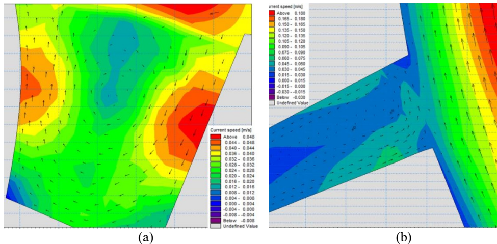
Fig. 15. Eddy currents in front of Tang Tang sluice (a) and in front of Ben Nghe sluice (b)
