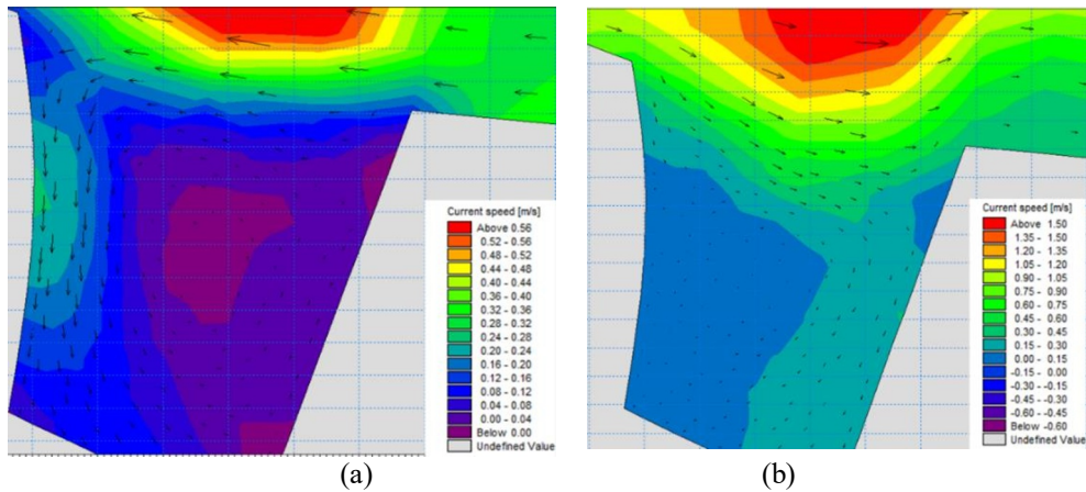
Fig. 13. Distribution of flow velocity in area of Tan Thuan sluice in high water at high tide (a) and low tide (b).
