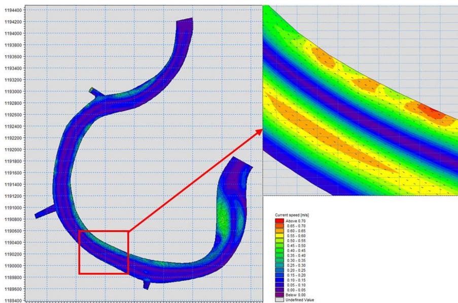
Fig. 14. Distribution of flow velocity at end of low tide to beginning of high tide.
