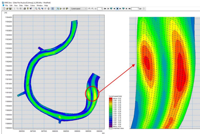
Fig. 9. Flow velocity distribution in initial phases of tide in April-May.
