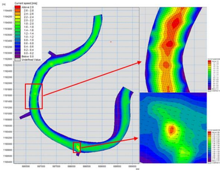
Fig. 7. Flow velocity field on Saigon River section at low tide.
