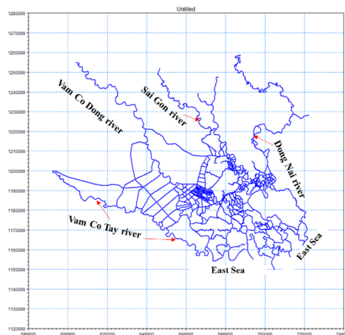
Fig. 3. Saigon – Dongnai River network on MIKE 11.
