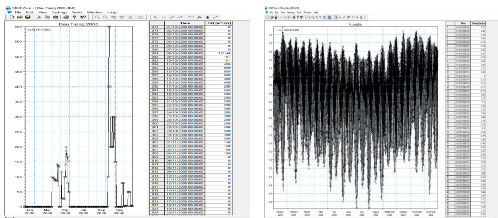
Fig. 5. Flood discharge of the Dau Tieng reservoir (a) and the water level in Vung Tau (b) in 2000
