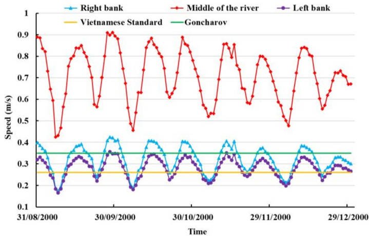
Fig. 16. Estimated flow velocity and non-erosive velocity
