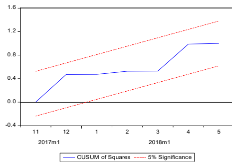
Fig. 2. The sum of squares of regressive residues (CUSUM of Squared) test
