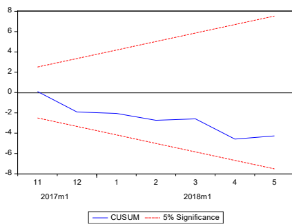
Fig. 1. Regressive residual sum test (CUSUM)
