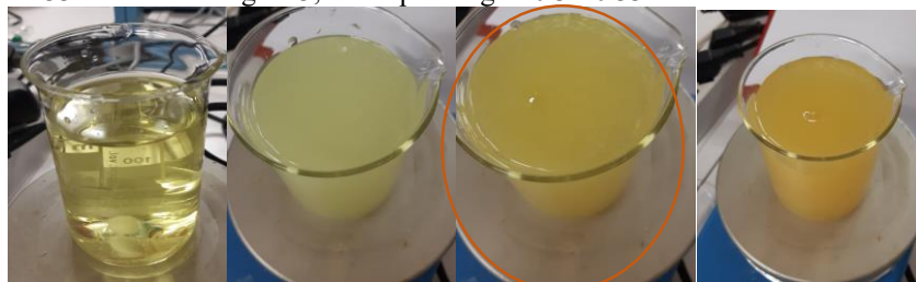
Fig. 3. Color change after the qualitative Mohr titration: initial (yellow) color for the presence of K_3Fe(CN)_6 indicator, yellow-opaque color after precipitation of 0.1mmol of AgCl , yellow-to-orange turning point @33ml of added 0.01M AgNO_3 (circled) and orange color for the Ag_3Fe(CN)_6 precipitates.
