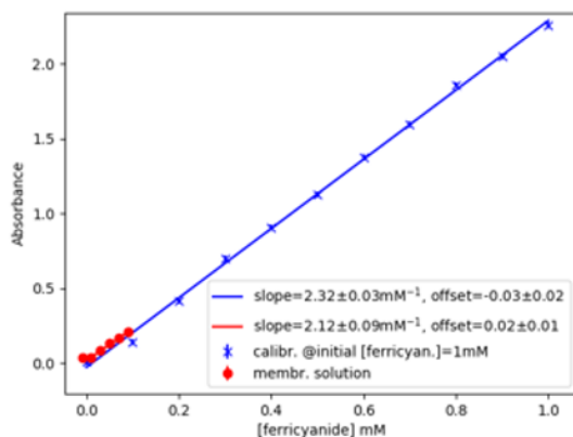
Fig. 1. Spectrophotometric assessment of absorbance as a function of ferricyanide concentration for the calibration solution with 1mM of initial K_3Fe(CN)_6 concentration (blue crosses) and the membrane solution (red dots). Concentrations decrease from right to left as long as ascorbic acid is added and K_3Fe(CN)_6 reduced to K_4Fe(CN)_6 .
