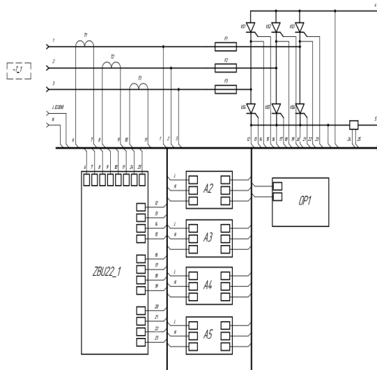
Fig. 3. Electrical circuit of battery management and control structure.
