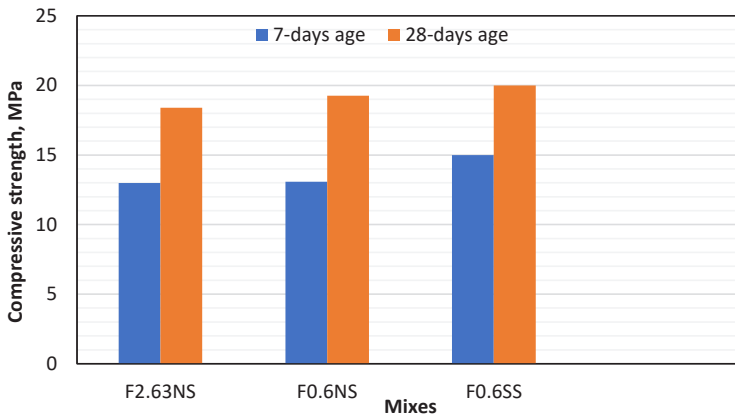
Figure 6: Compressive strength results for all mixes.
