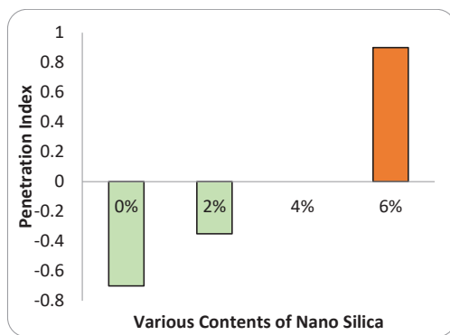
Figure 6: Penetration index and % nano silica.
