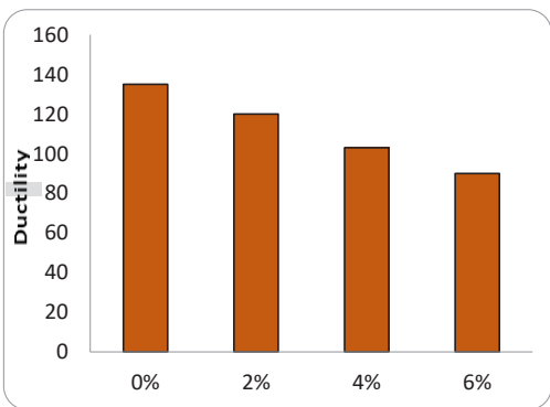
Figure 8: Ductility and % nano silica.
