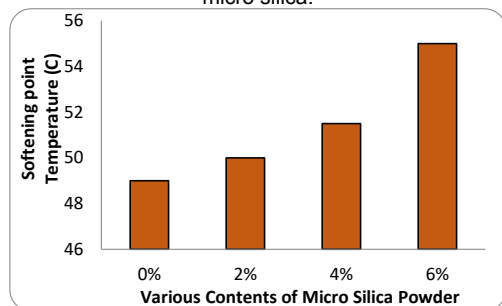
Figure 3: Softening point temperature and % micro silica.
