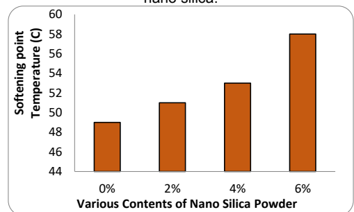
Figure 4: Softening point temperature % nano silica.
