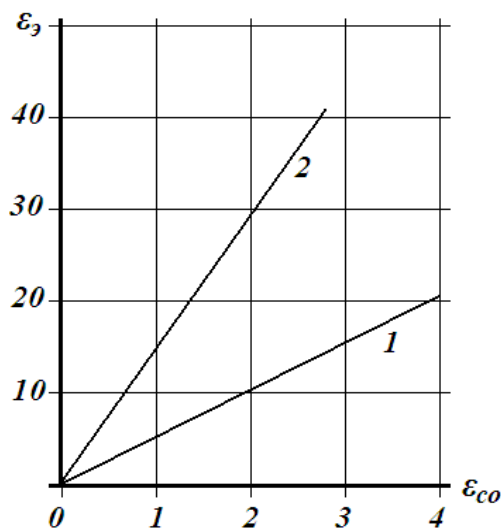
Fig. 5. Dependences \epsilon_3 = f(\epsilon_{co}) corresponding to the condition \epsilon_c \cos^2 \psi_c = 0,05 \epsilon_3 \cos^2 \psi_3 with (1) and without (2) nonlinear properties of the steel mass.
