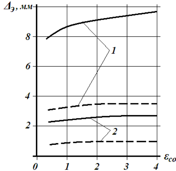
Fig. 4. Dependences of the thickness of the aluminum (1) and copper (2) screens of the combined SE on \epsilon_{co} , corresponding to the condition \epsilon_c \cos^2 \psi_c = 0,05 \epsilon_3 \cos^2 \psi_3 . Inductor linear load: 5 \times 10^4 A/m (solid lines) and 0.5 \times 10^4 A/m (dashed lines).
