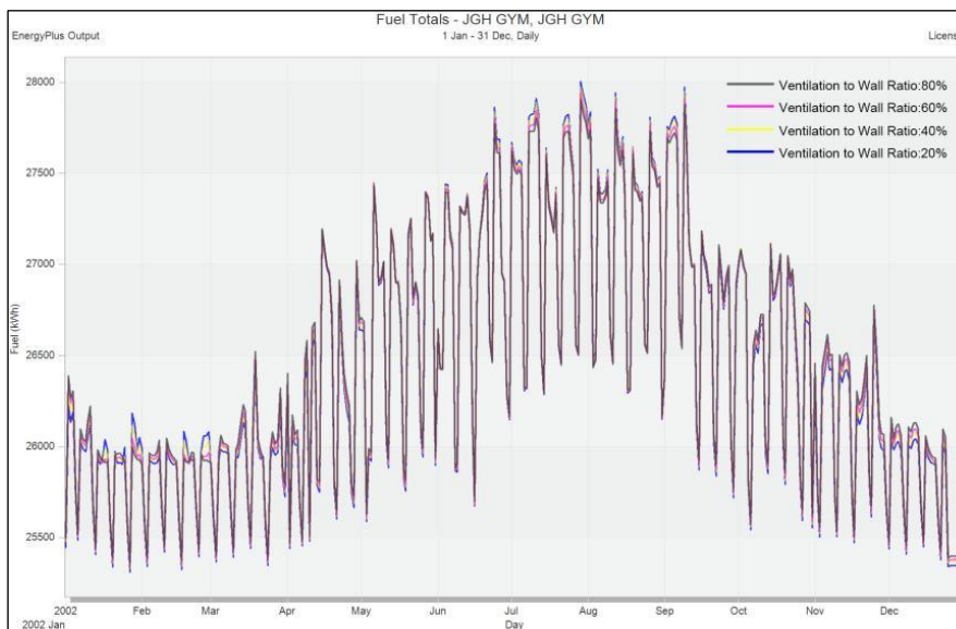
Figure 6. Energy consumption for different ventilation-to-wall ratios.
