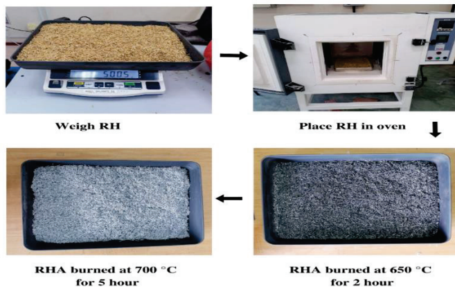
Fig. 3 process of controlled combustion of RH.
