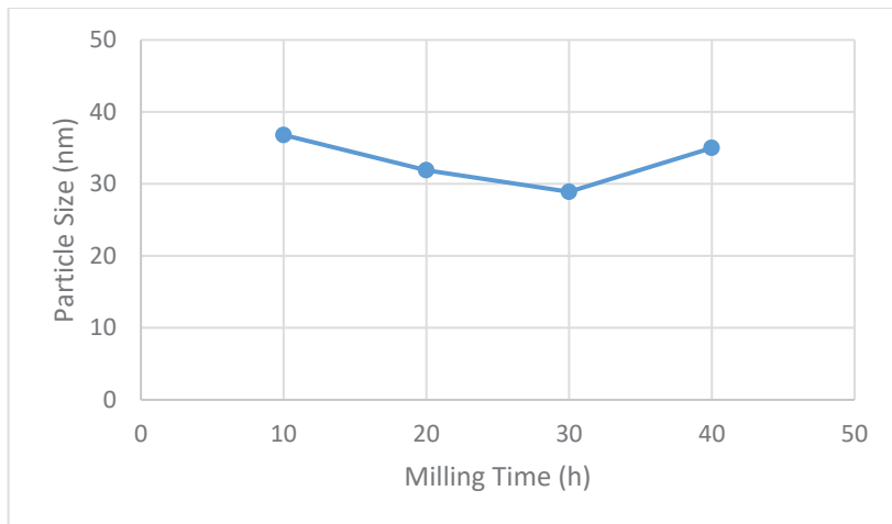
Fig. 6. Effect of grinding time on the mean particle size of nano RHA
